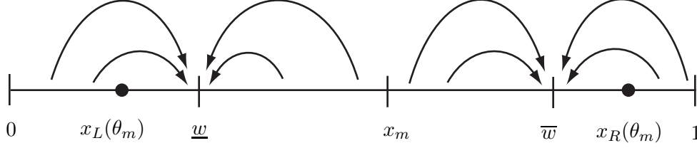
Figure 3: Strongly partisan equilibrium
